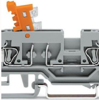
Wago Disconnect Terminal 2-Way along with accessories
