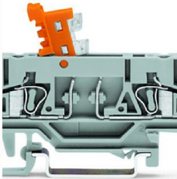
Wago Disconnect Terminal 4-Way along with accessories
